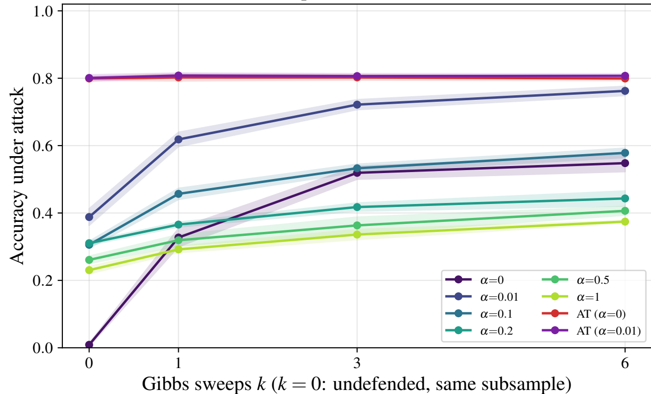
d3r10c64 — Gibbs purification ( \varepsilon = 0.2 , n_{\text{eval}} = 250 )
