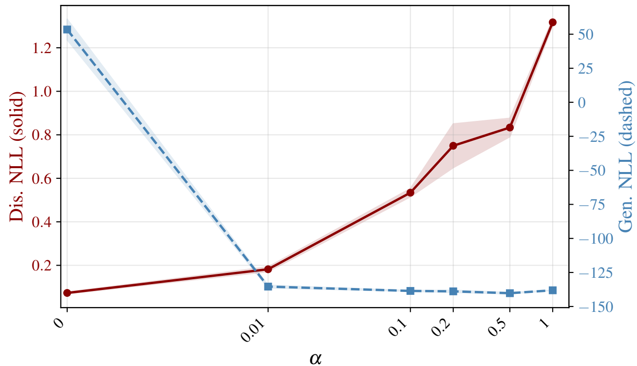
d3r20c64 — NLL vs \alpha
