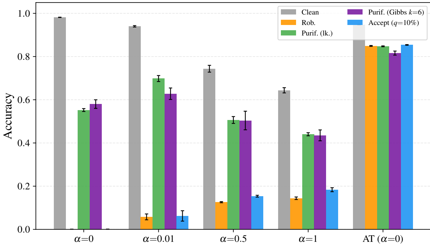
d3r40c64 — defenses at \varepsilon = 0.3
