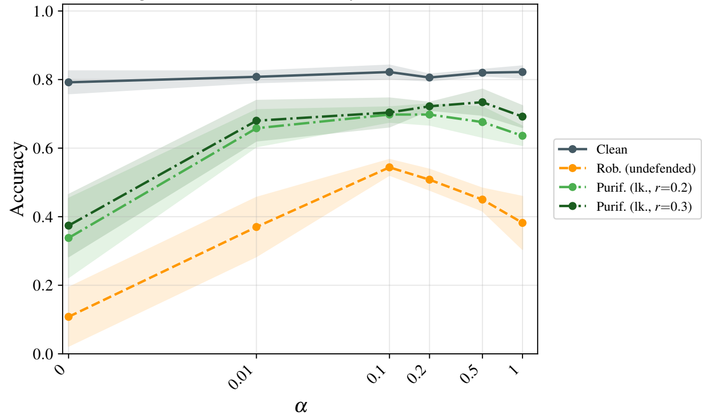
ecg200 d3r10c64 — accuracy vs \alpha ( \epsilon = 0.2 )
