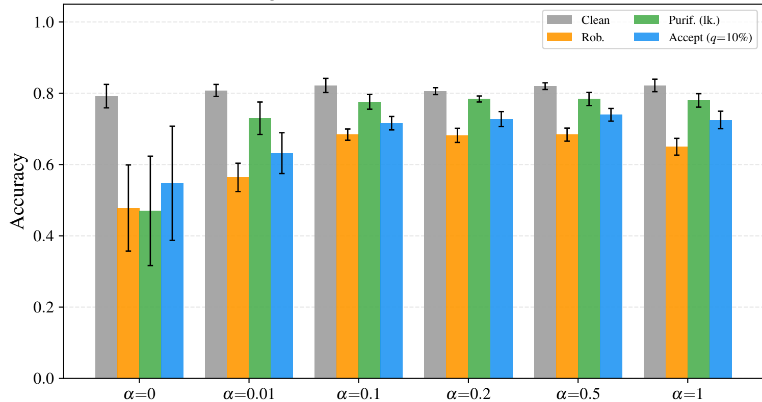
ecg200 d3r10c64 — defenses at \varepsilon = 0.1
