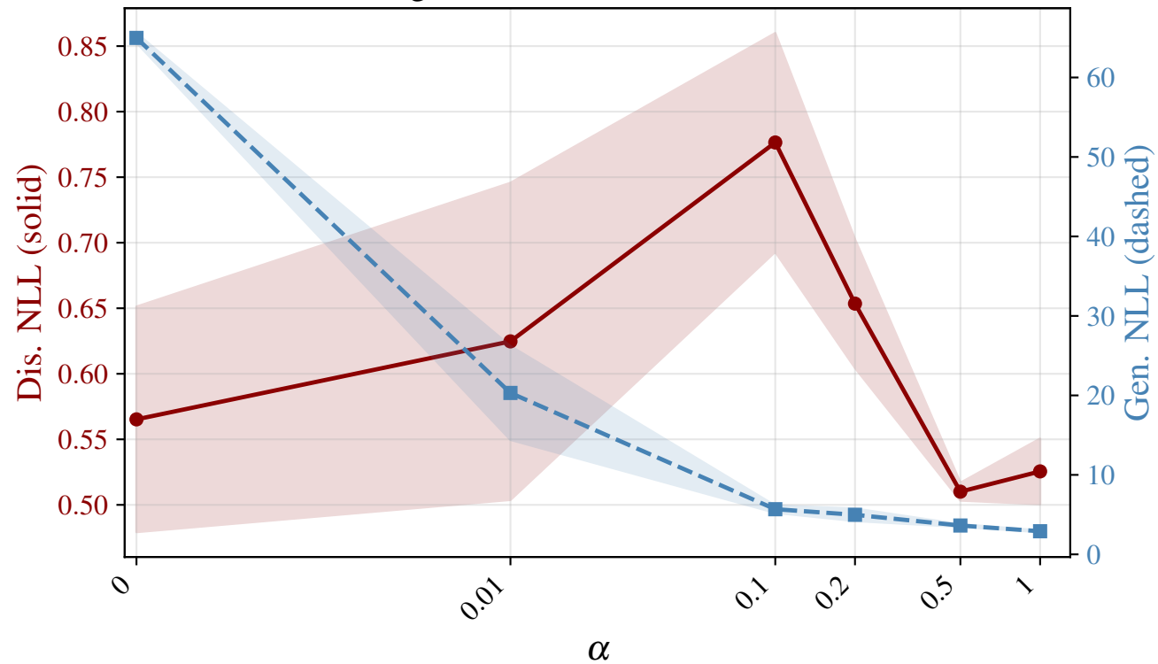
ecg200 d3r20c64 — NLL vs \alpha
