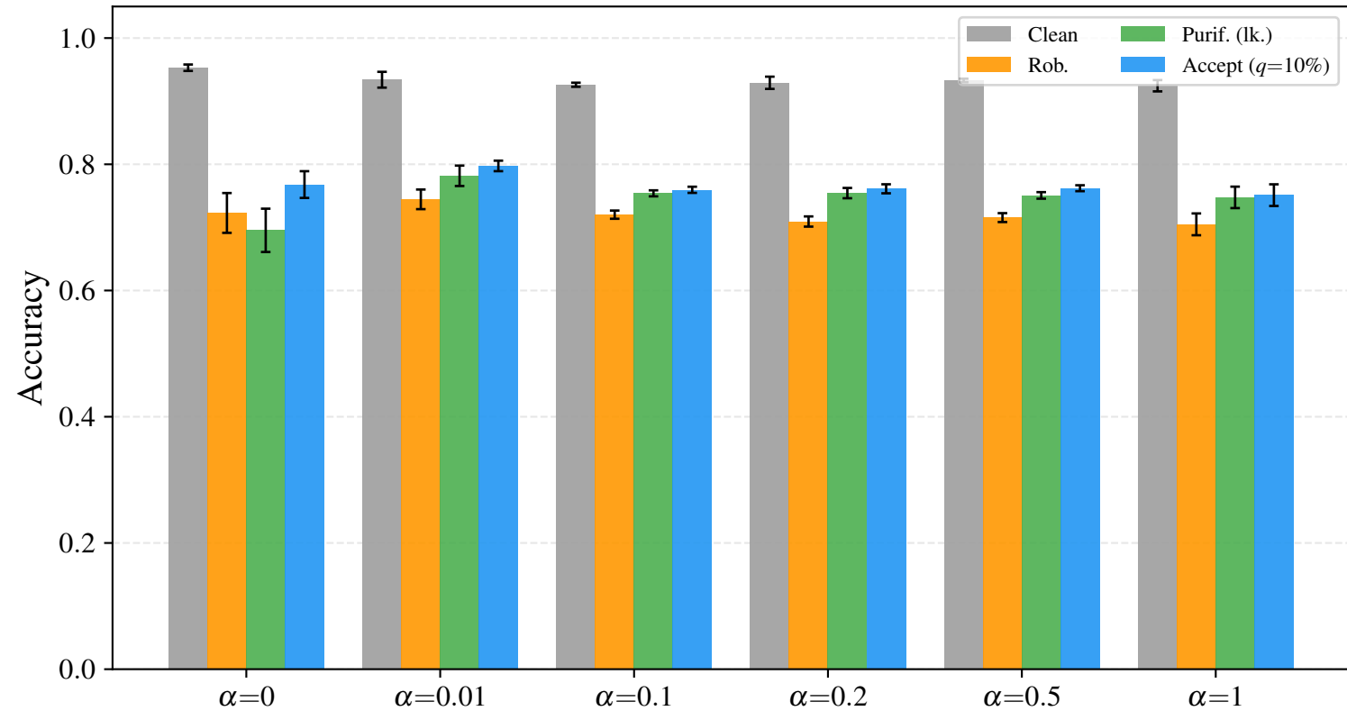
itilypowerdemand d3r20c64 — defenses at \epsilon = 0.1
