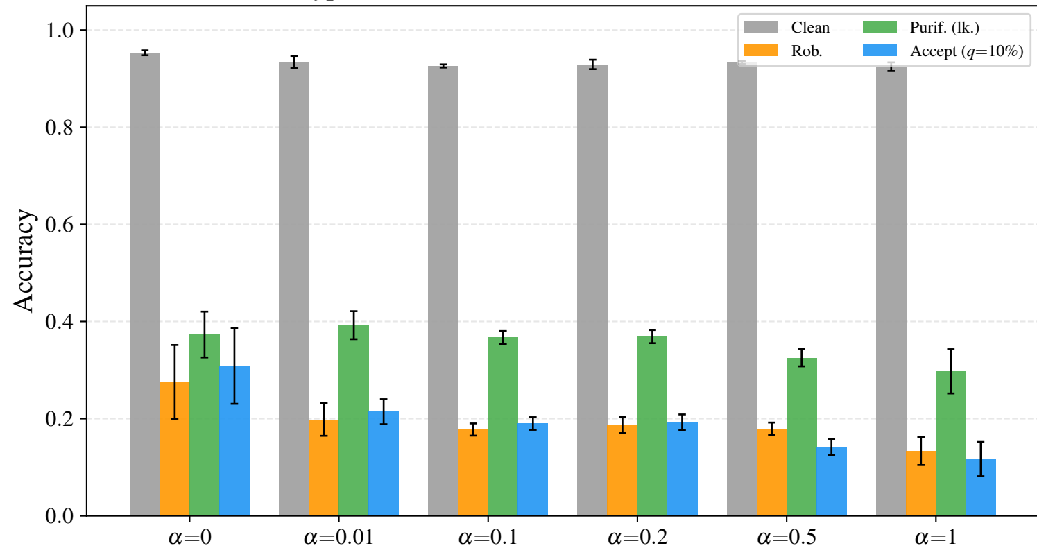
italypowerdemand d3r20c64 — defenses at \epsilon = 0.3
