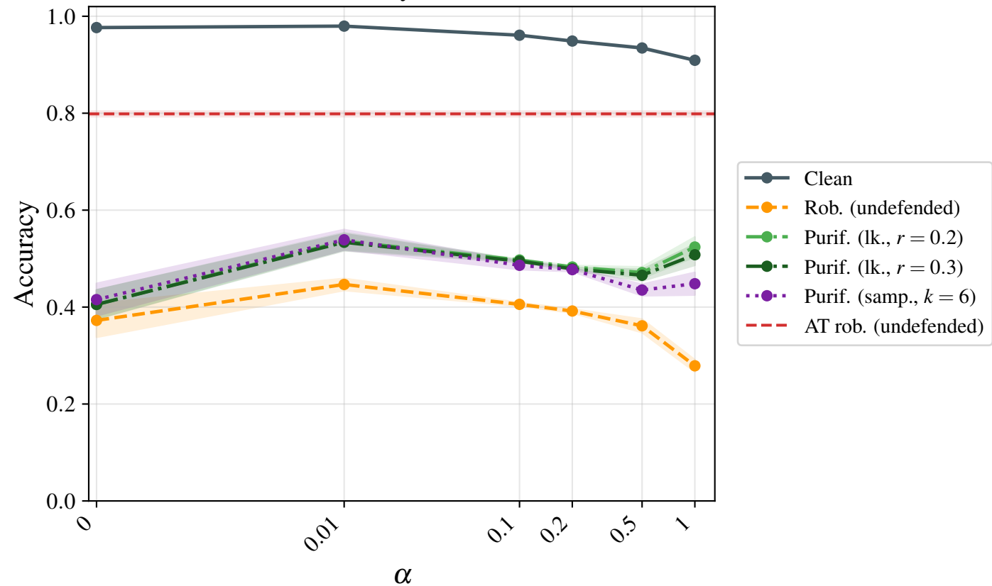
JEM — accuracy vs \alpha ( \epsilon = 0.2 )
