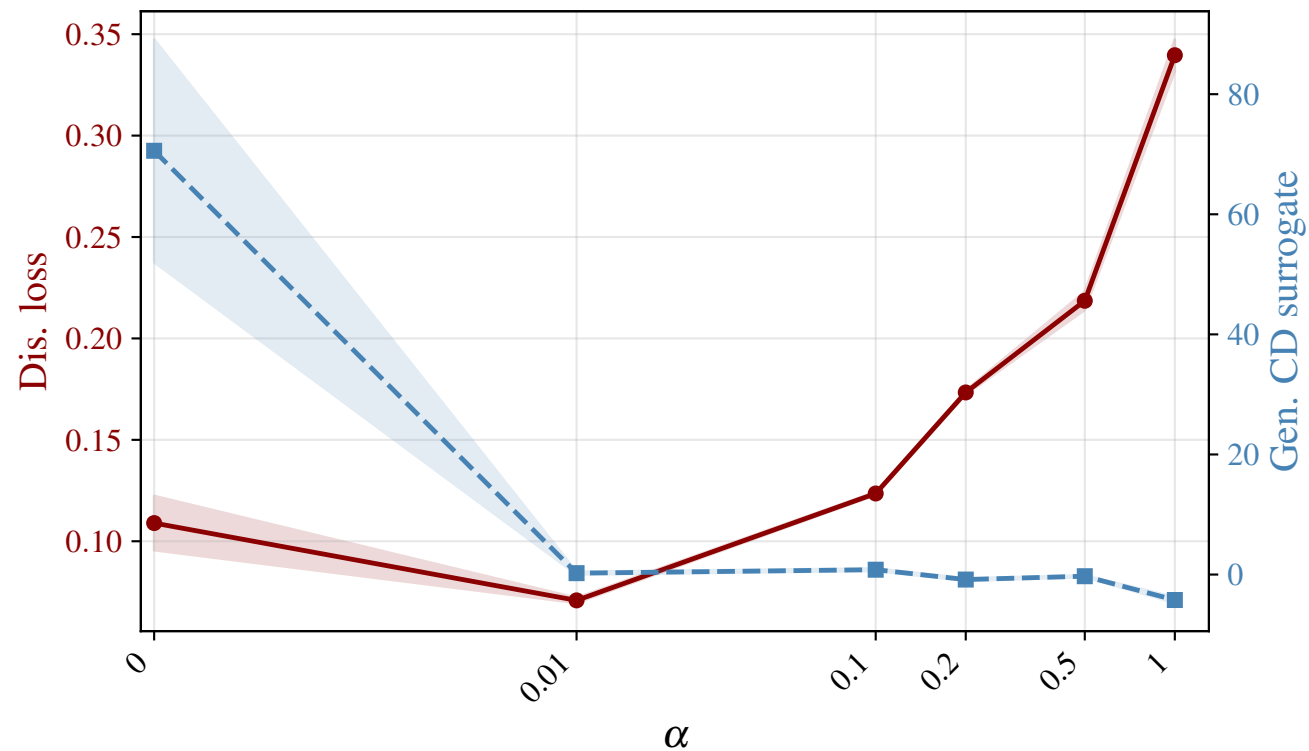
JEM — losses vs \alpha
