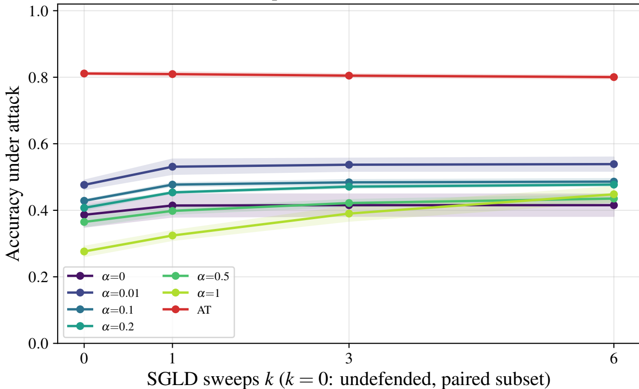
JEM — SGLD purification ( \epsilon = 0.2 , n_{eval} = 1000 )
