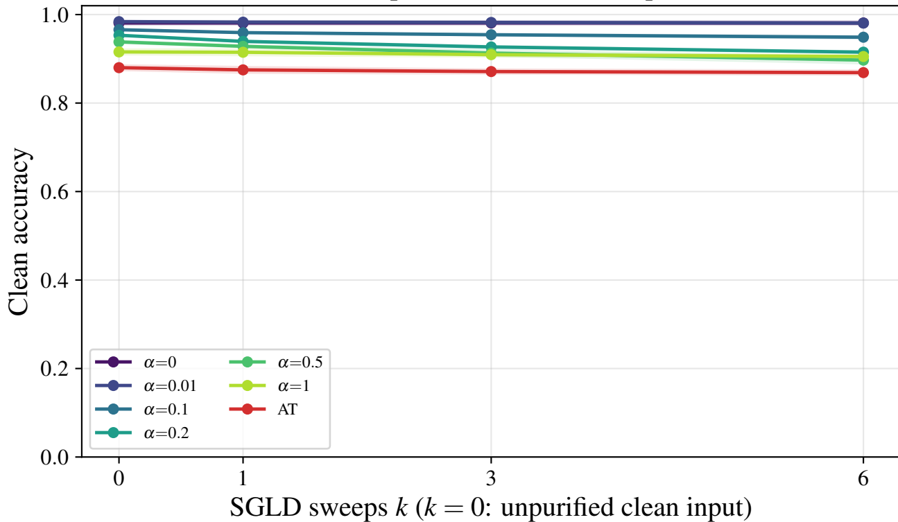
JEM — cost of SGLD purification on clean input ( n_{eval} = 1000 )
