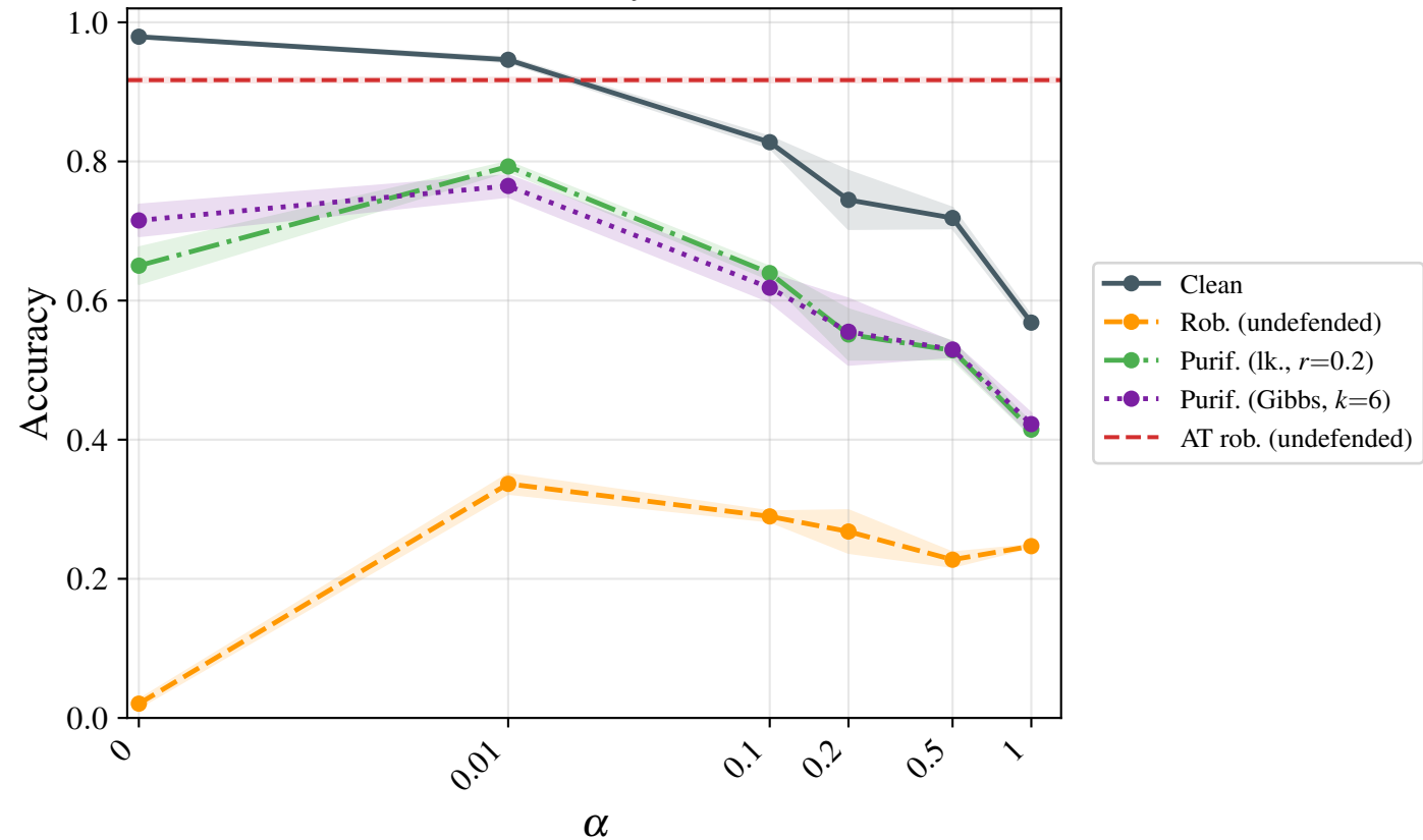
d3r20c64 — accuracy vs \alpha ( \epsilon = 0.2 )
