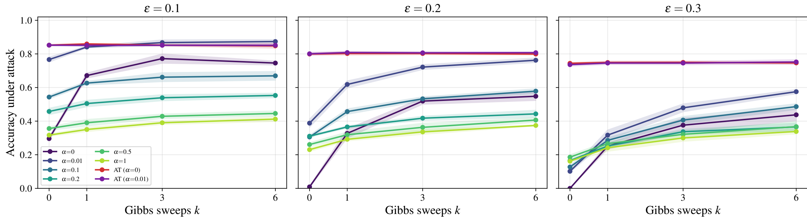
d3r10c64 — Gibbs purification vs k ( n_{\text{eval}} = 250 )
