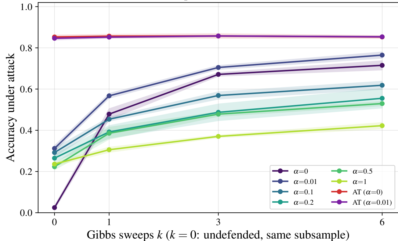
d3r20c64 — Gibbs purification ( \varepsilon = 0.2 , n_{\text{eval}} = 250 )
