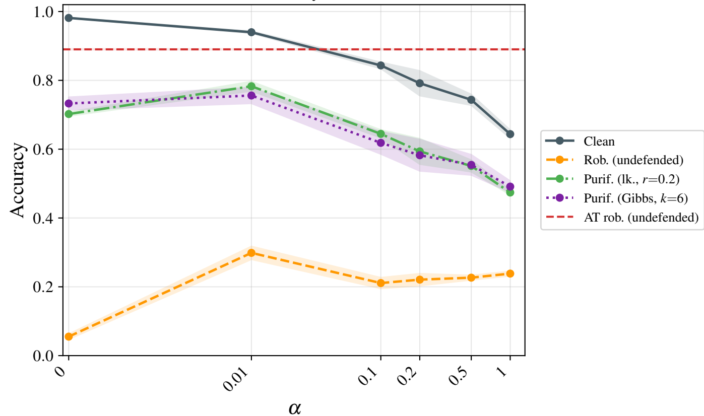
d3r40c64 — accuracy vs \alpha ( \epsilon = 0.2 )
