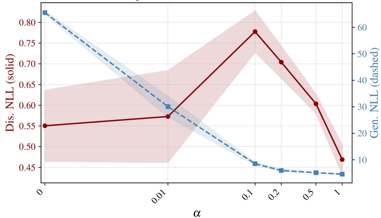
ecg200 d3r10c64 — NLL vs \alpha
