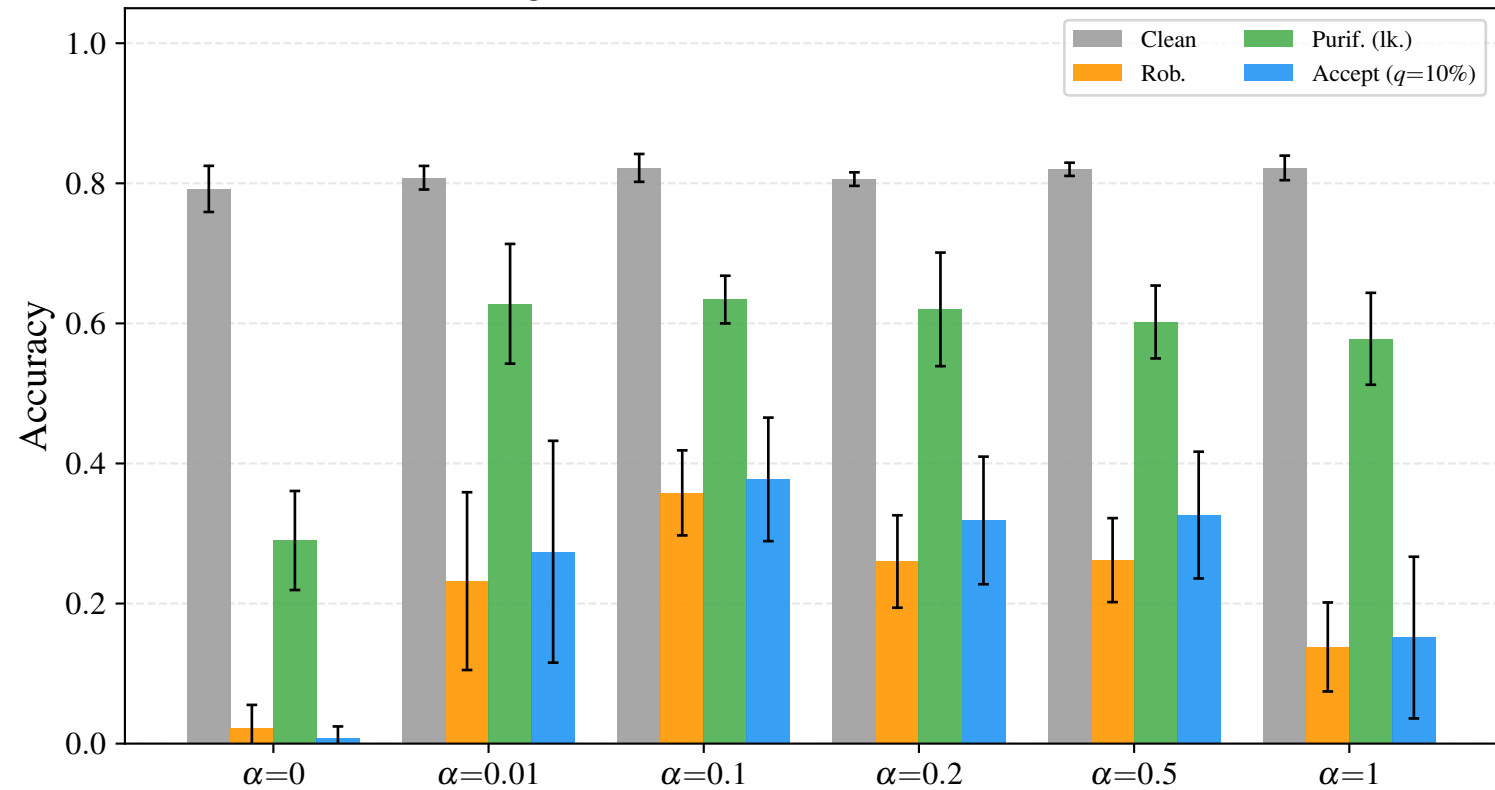
ecg200 d3r10c64 — defenses at \epsilon = 0.3
