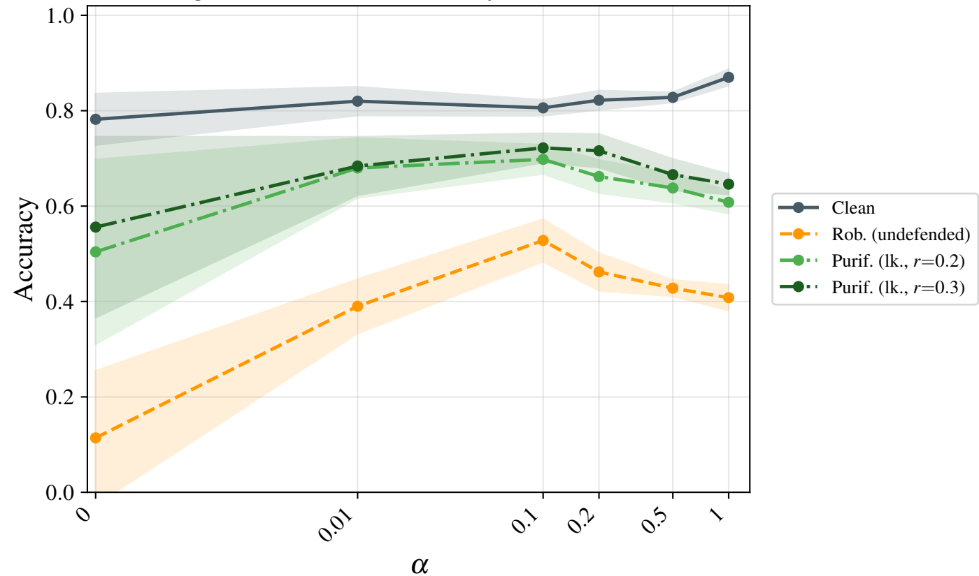
ecg200 d3r20c64 — accuracy vs \alpha ( \epsilon = 0.2 )
