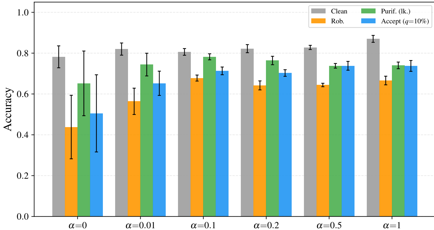
ecg200 d3r20c64 — defenses at \varepsilon = 0.1
