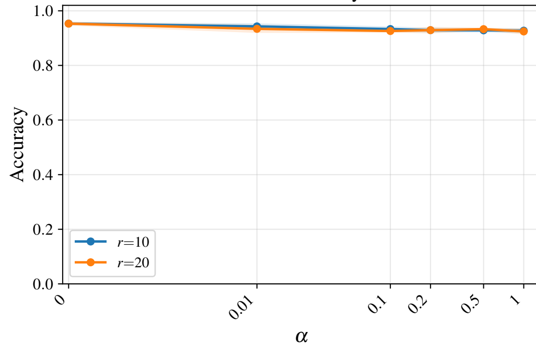
Clean accuracy
