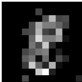
purified \alpha = 0.1
