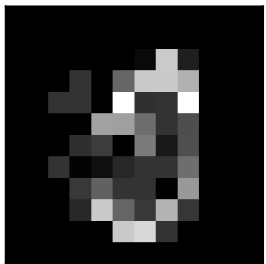
adversarial
