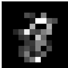
AT-model purified
