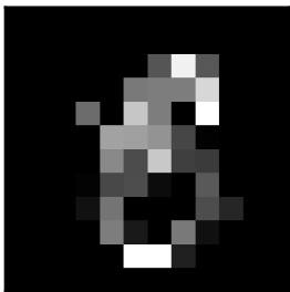
purified \alpha = 0.01
