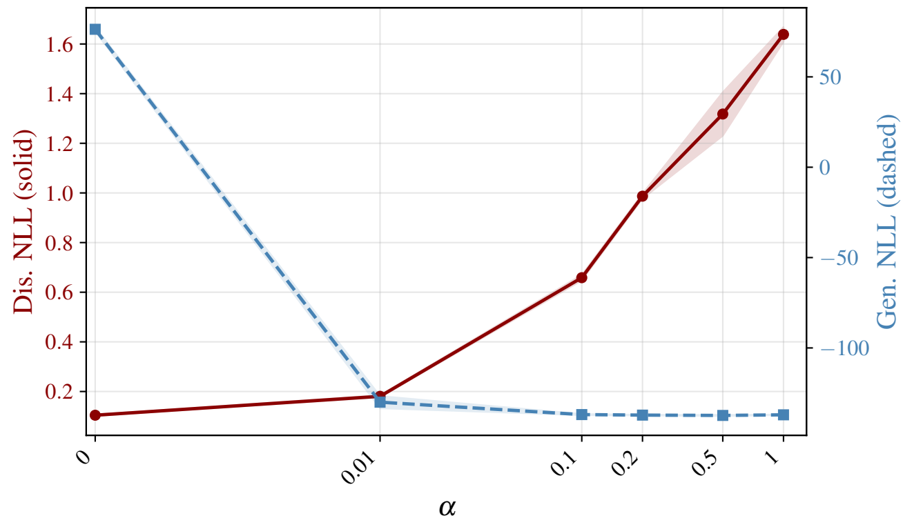
d3r10c64 — NLL vs \alpha
