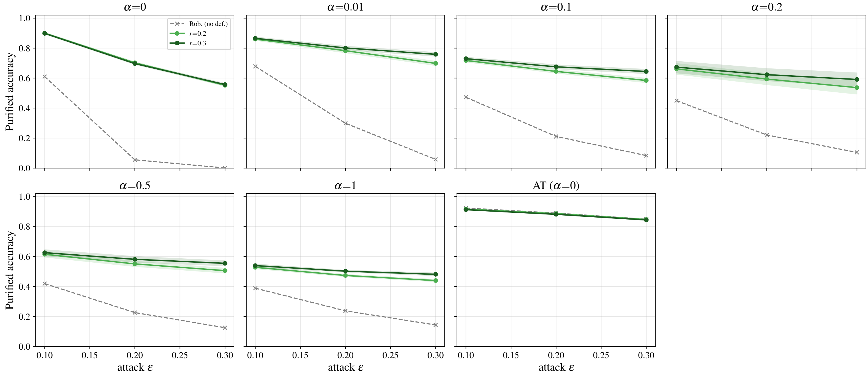
d3r40c64 — likelihood purification radius
