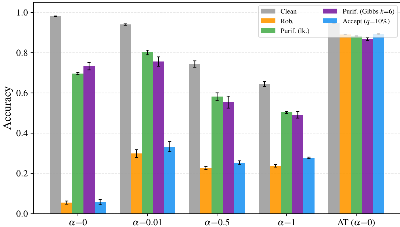
d3r40c64 — defenses at \varepsilon = 0.2
