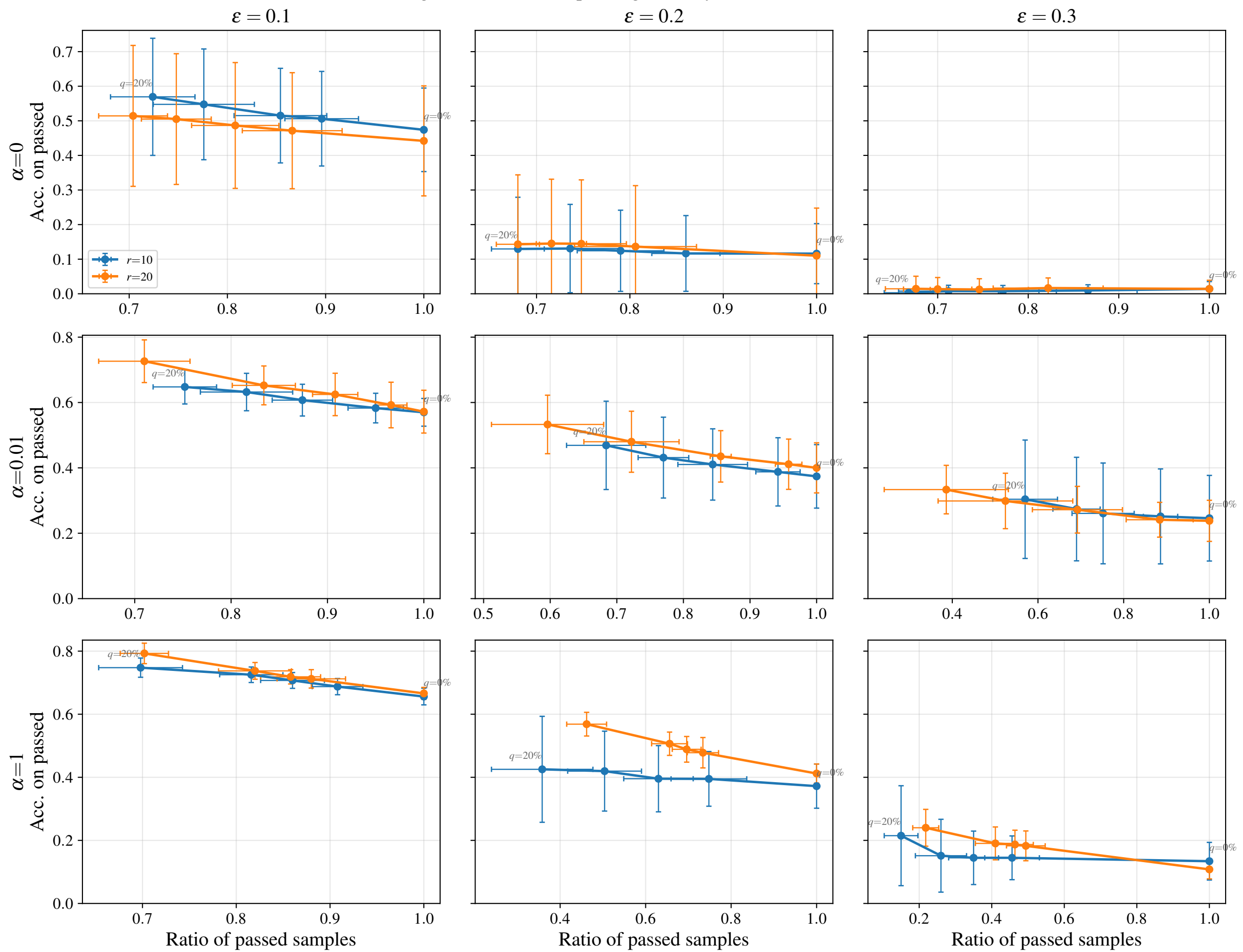
ecg200 — detection operating curve by bond dimension
