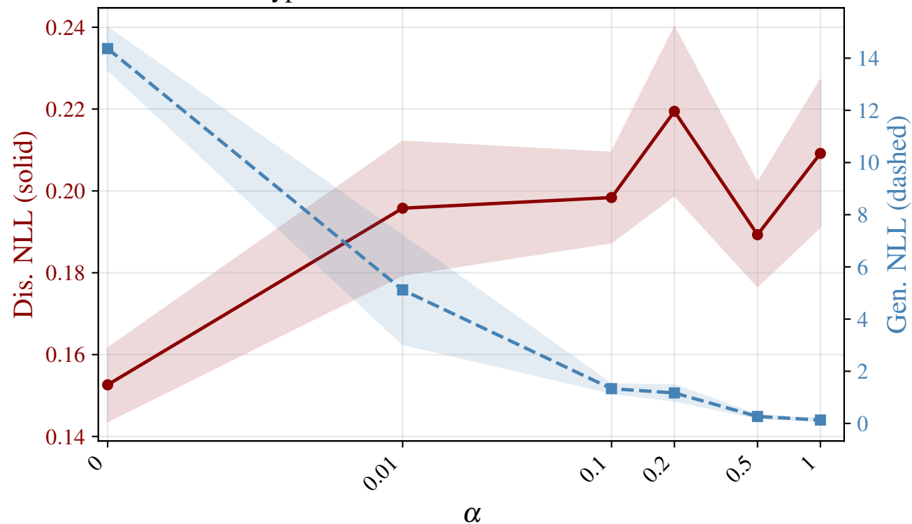
italypowerdemand d3r10c64 — NLL vs \alpha
