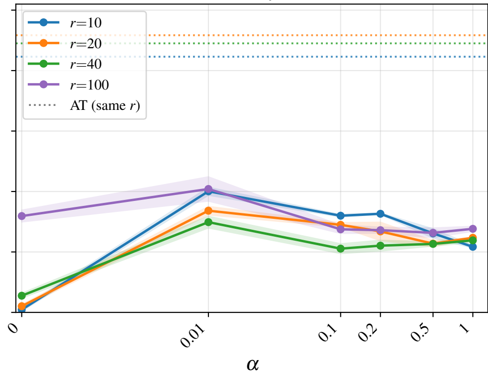
Robust accuracy ( \epsilon = 0.2 )
