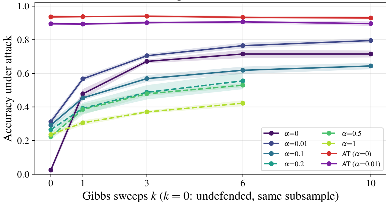
d3r20c64 — Gibbs purification ( \epsilon = 0.2 , n_{\text{eval}} = 250 )
