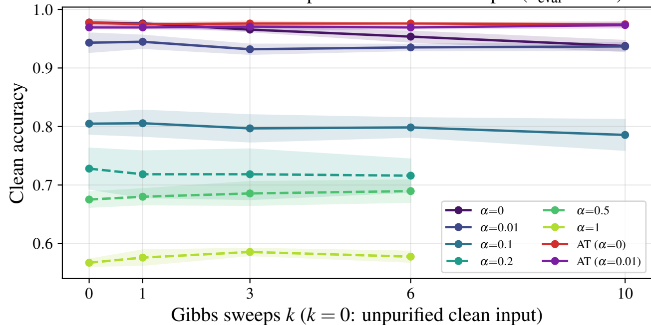
d3r20c64 — cost of Gibbs purification on clean input ( n_{\text{eval}} = 250 )
