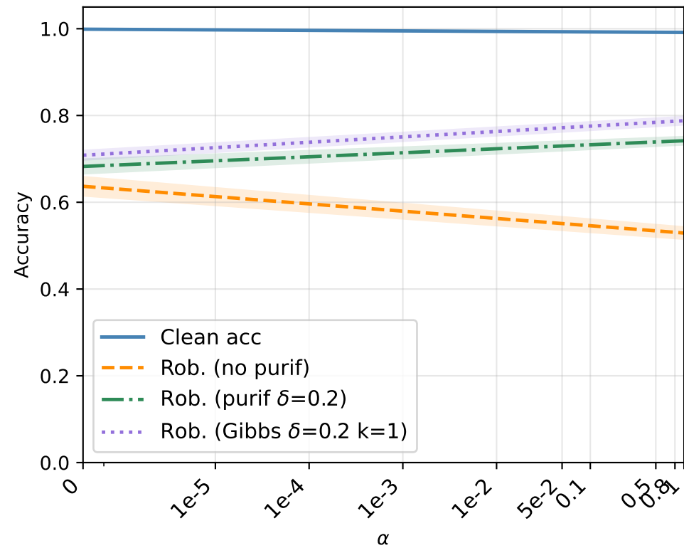
Accuracy vs \alpha ( \varepsilon = 0.2 )
