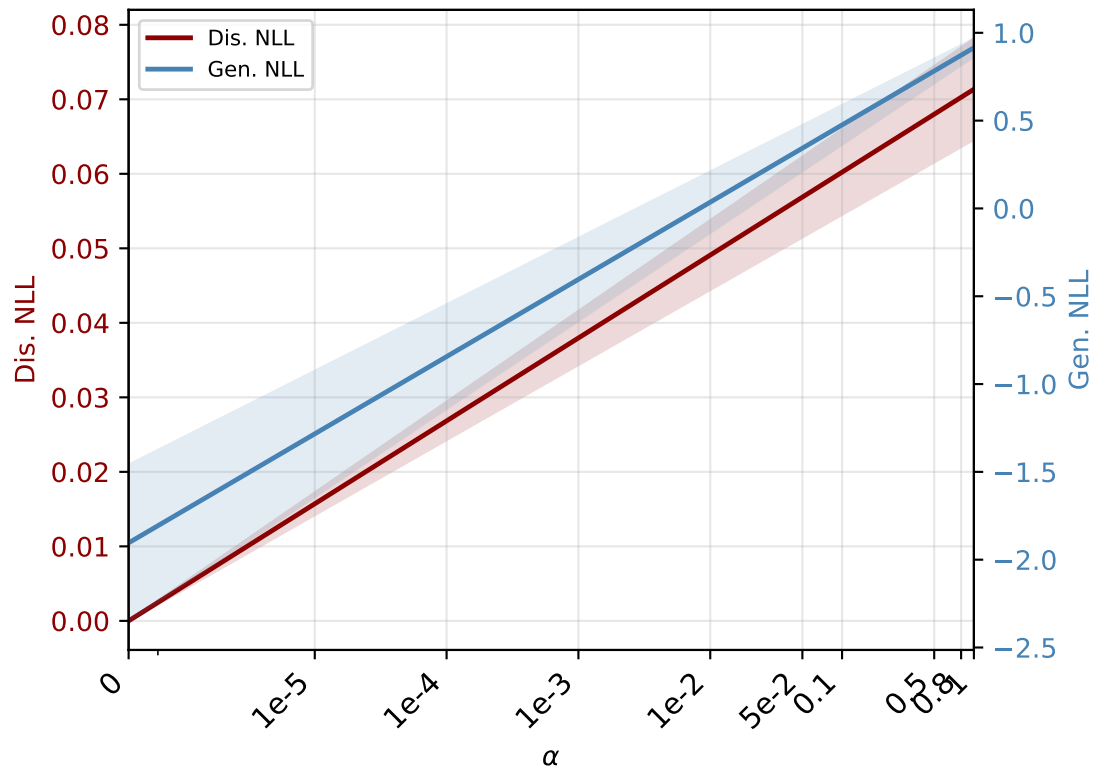
NLL Loss vs \alpha
