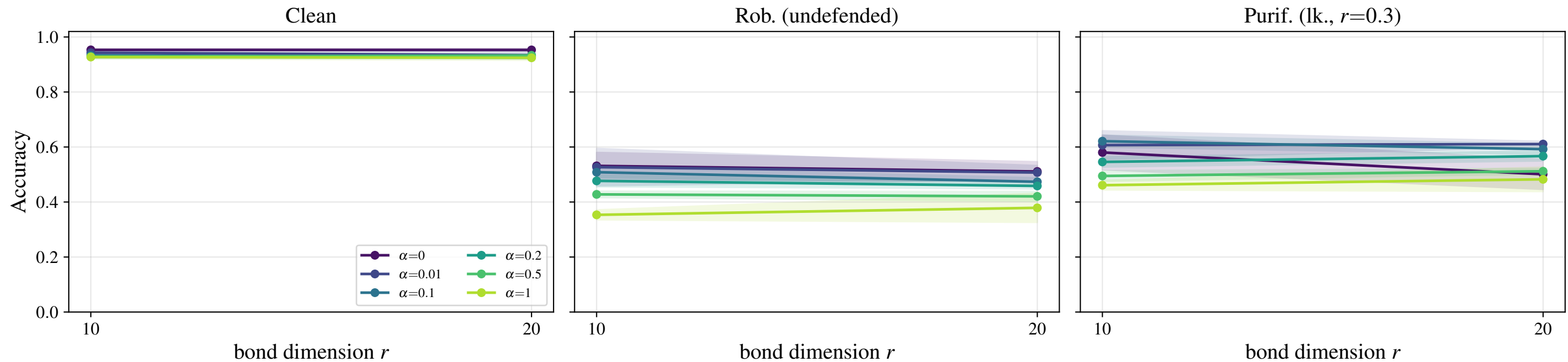
italypowerdemand — metrics vs bond dimension ( \varepsilon = 0.2 )
