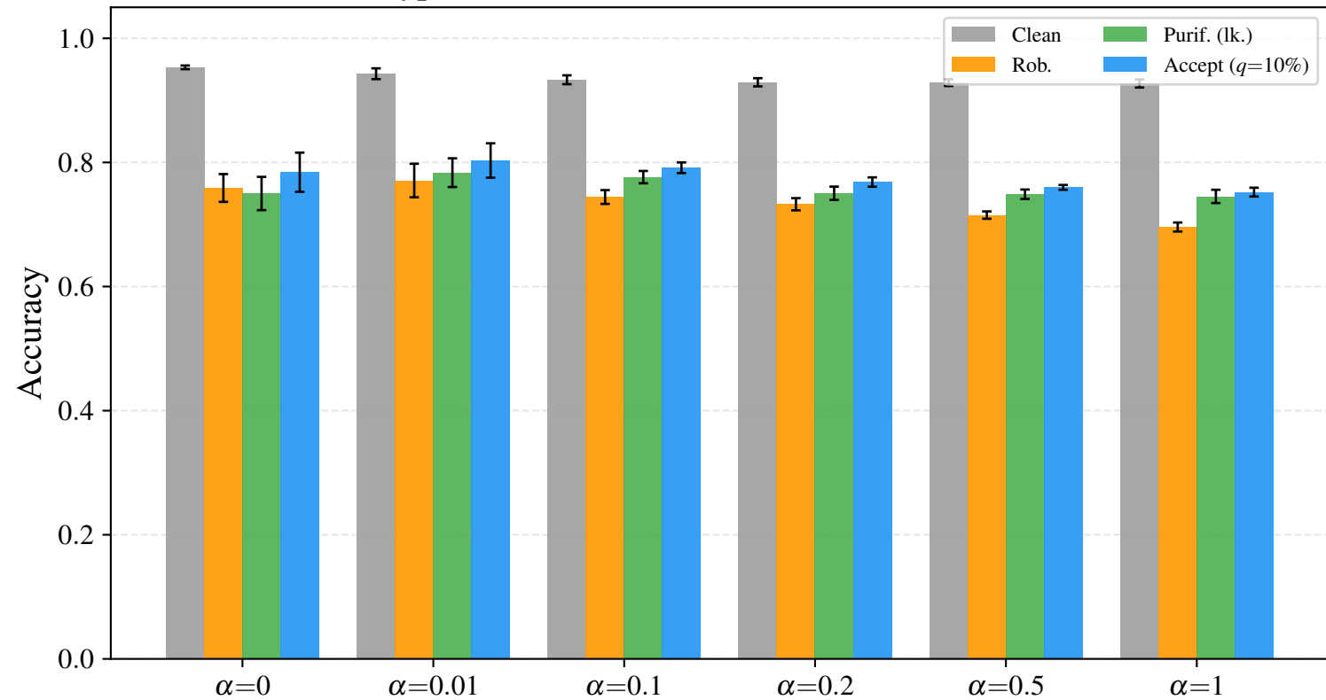
italypowerdemand d3r10c64 — defenses at \epsilon = 0.1
