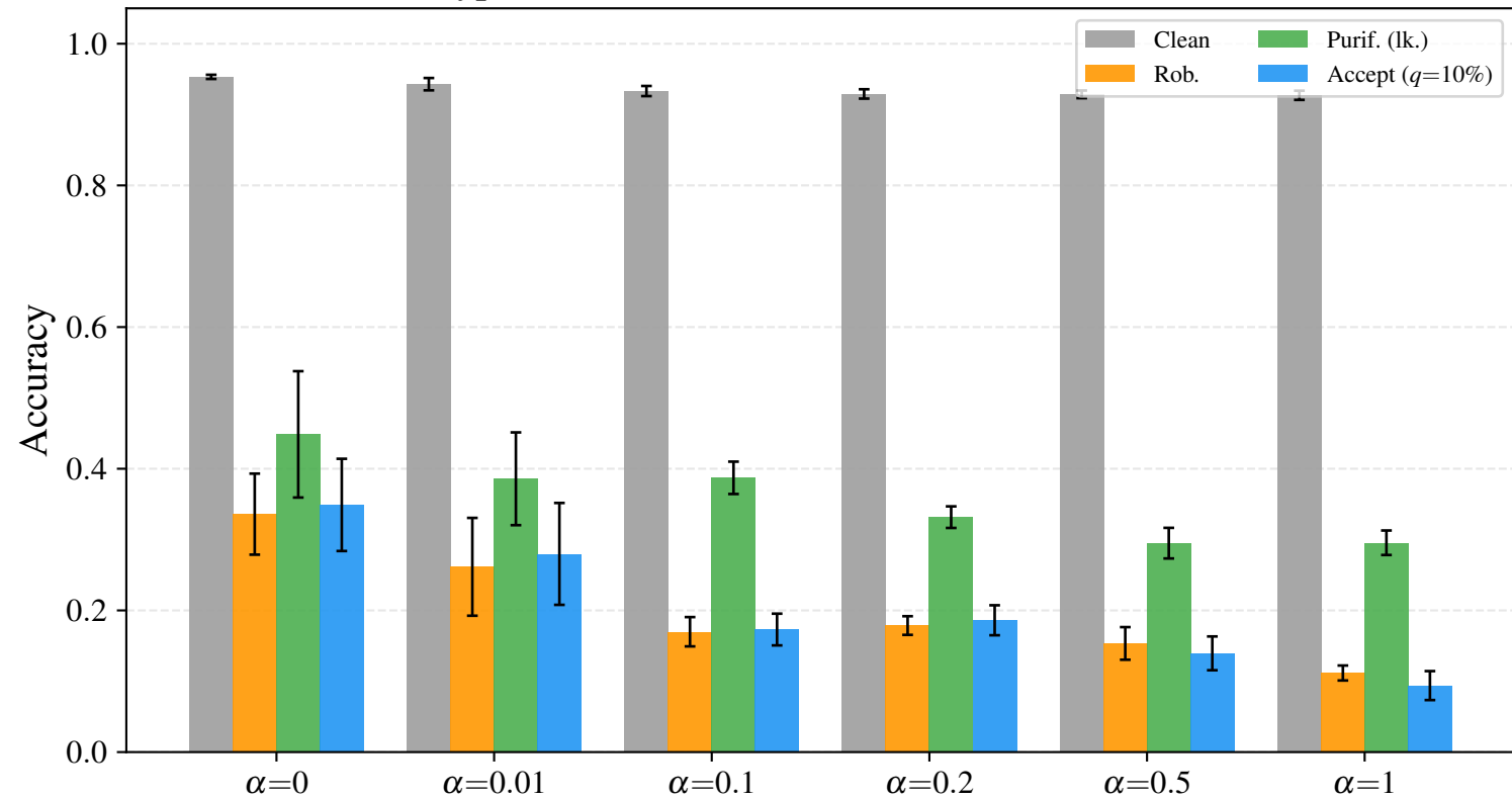
italypowerdemand d3r10c64 — defenses at \varepsilon = 0.3
