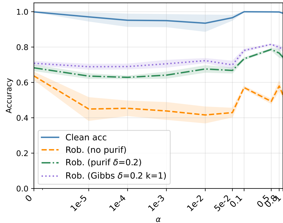
Accuracy vs \alpha ( \epsilon = 0.2 )
