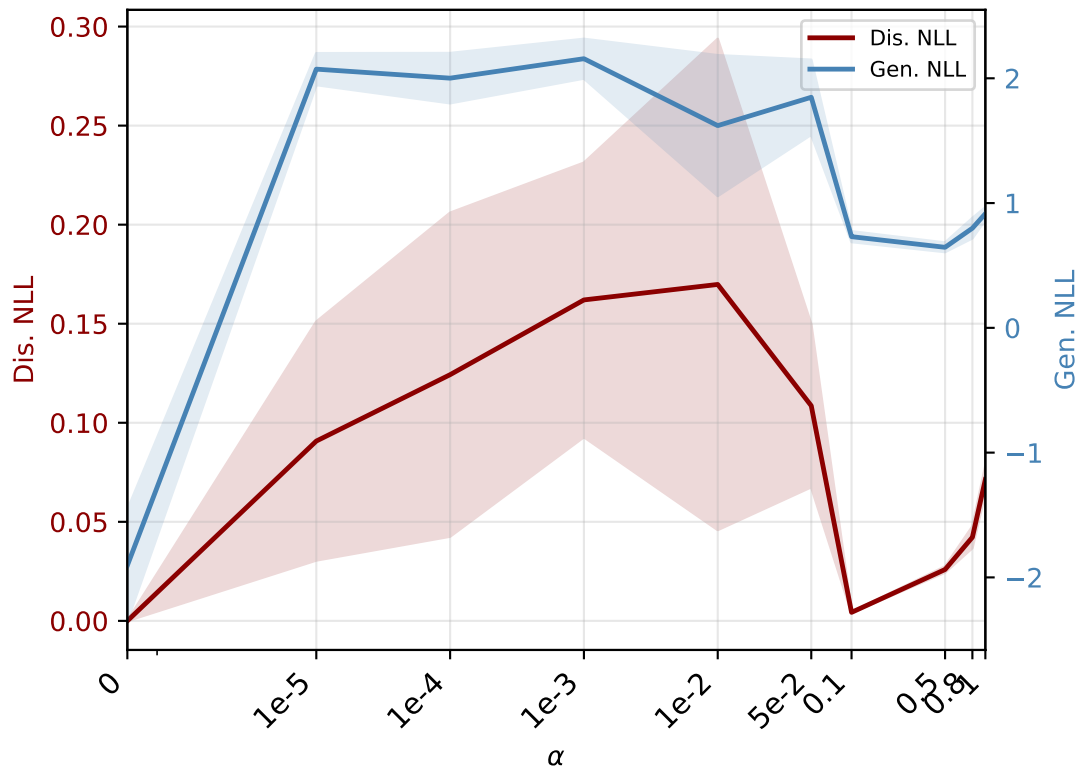
NLL Loss vs \alpha
