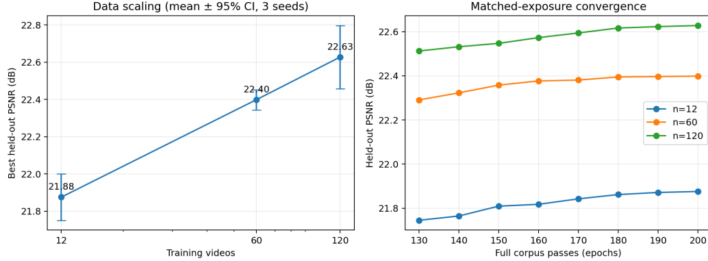
Figure 3: Support-correct encoder scaling. Left: held-out PSNR against training-set size, mean and 95% t interval over three seeds. Right: convergence against matched corpus exposure. The result is monotonic across these three small training sets.
