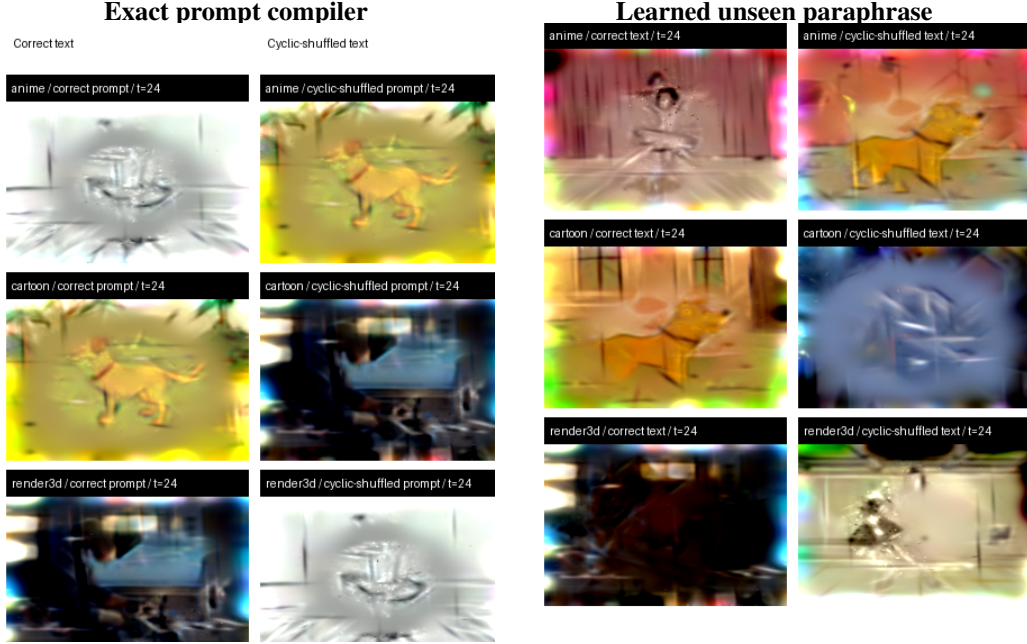
Figure 4: Prompt-only evidence sheet reflowed from one audited image. Each half shows correct-prompt and cyclic-shuffled generation for ballerina, dog, and welder classes. All evaluated samples are shown. These are 72k-Jewel renders, not source frames; their trajectory macro tokens are nevertheless backed by fitted training fields.
