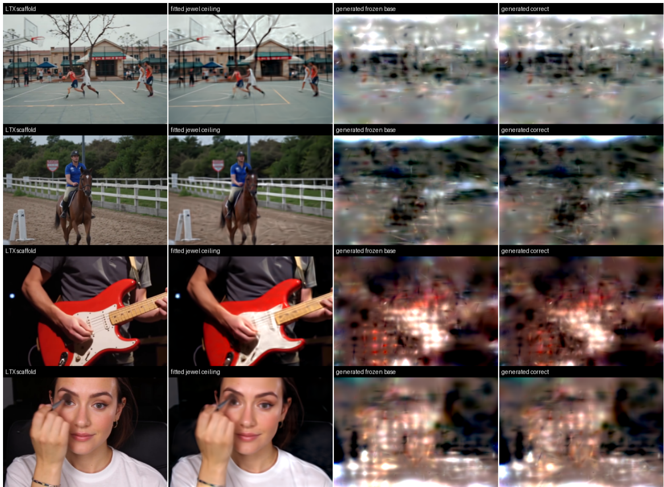
Figure 14: Exact-count native audit at the third-window frontier. The coupled field (right) shares every birth cell/rank and noise seed with the frozen base (center-right). Changes are real but subtle relative to the large gap to the fitted-field ceiling.
