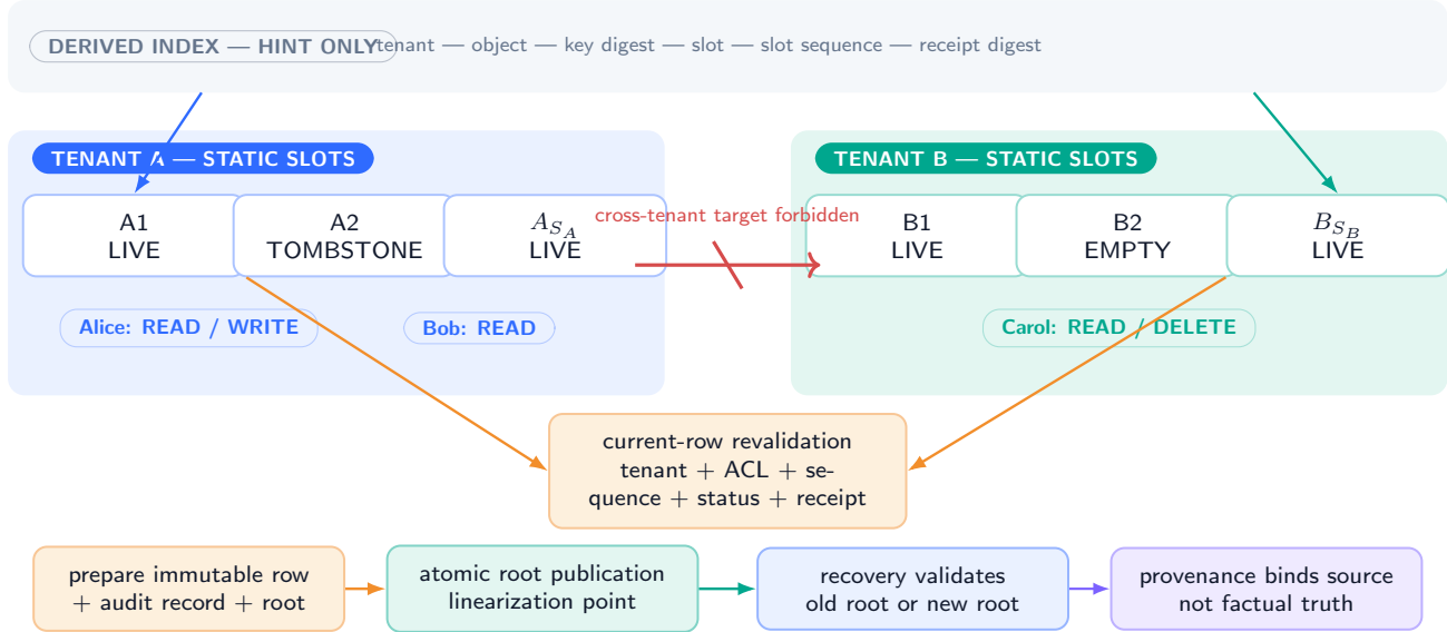
Figure 32: Static tenant partitions, system-owned security, and current-row revalidation define the logical boundary. Indexes are hints, provenance binds declared sources, and publication binds the row to an audit root. The proved path excludes side channels and depends on authenticated context, serializable checks, and crash-safe storage assumptions.
