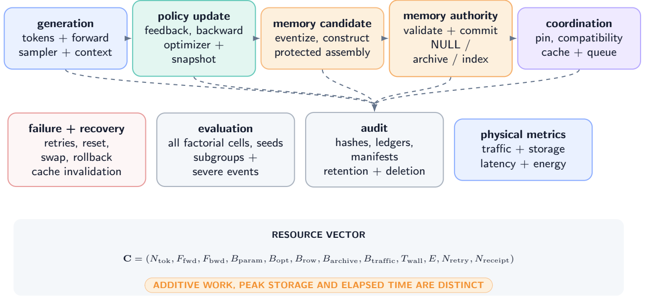
Figure 53: Training, reasoning-time, memory, recovery, and audit ledgers (DEFINITION / DESIGN PRESCRIPTION). Parallelism may reduce wall time but cannot delete logical work, bytes, validation, or failed attempts from the ledger.
