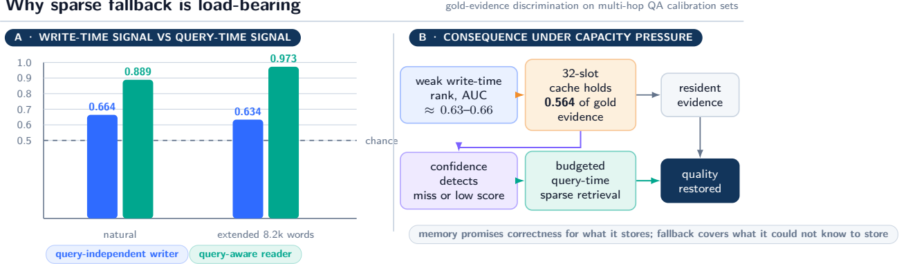
Figure 11: Gold-evidence discrimination on calibration questions. Passage-only features provide little information about which evidence a future question will need. Once the question is available, the same selection problem becomes much easier. A bounded writer therefore needs an explicit way to abstain and retrieve at query time.
