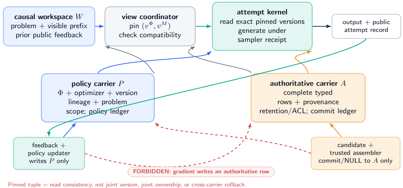
Figure 46: Typed dual-state architecture (DEFINITION / UNVALIDATED) . The attempt kernel reads a pinned view. Feedback may drive a policy update; a separate trusted path may assemble and commit a complete row. Dashed coral paths are forbidden privilege crossings.
