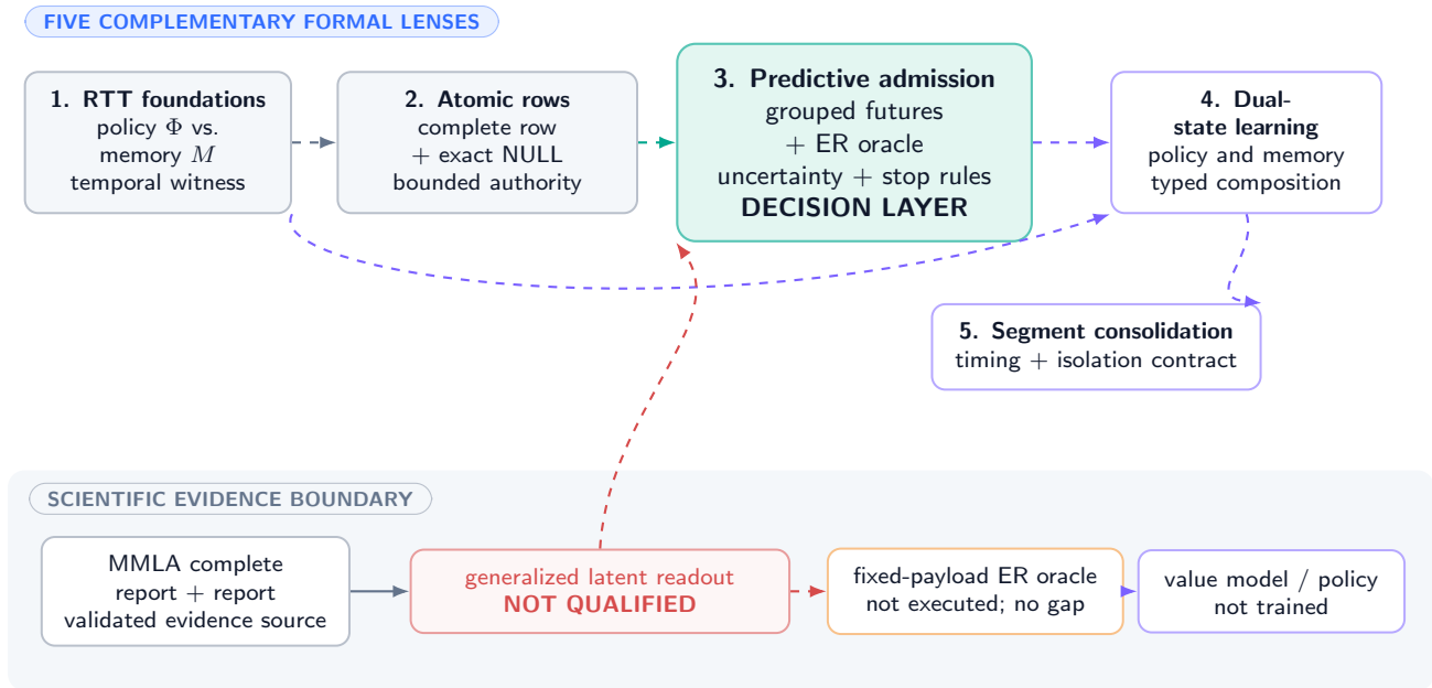
Figure 35: Predictive memory admission: future-valued action selection and the distinction between a conditional oracle target and an empirically established advantage.
