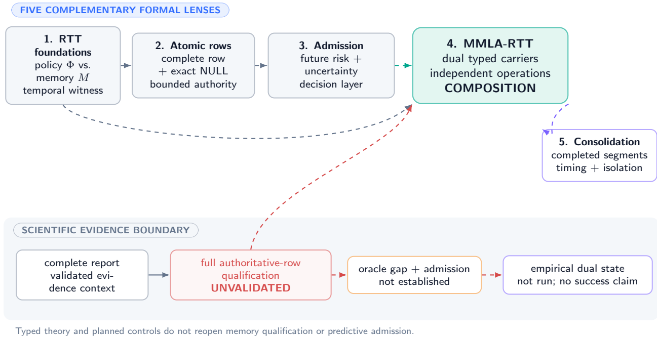
Figure 45: Dual-state composition: separate policy and memory carriers, their coordination, and the independently required evidence for a joint benefit.
