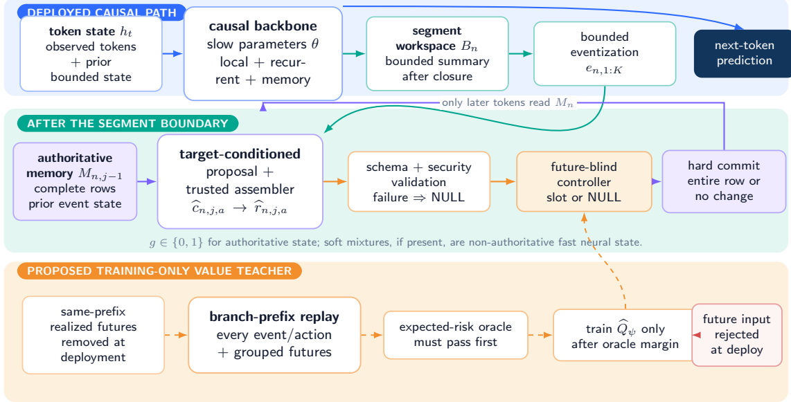
Figure 3: Predictive memory consolidation. The language model predicts causally and reads only prior persistent state. After a local segment is complete, a bounded bidirectional consolidator may reinterpret that observed segment and emit ordered events. At training time, several realized continuations with the same prefix estimate the conditional risk of every registered event-level action. A causal value model regresses those risks. At deployment the continuation branches are absent; one complete row is overwritten or NULL leaves state unchanged per event, and only later tokens read the resulting segment state.
