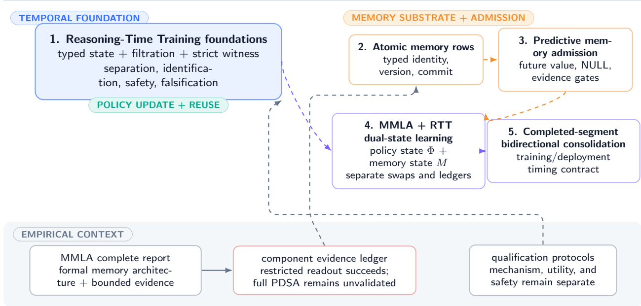
Figure 15: Reasoning-time training: the within-problem policy mechanism, its causal witness, and its relationship to the other theory divisions. Conditional results do not constitute an executed policy-only intervention.
