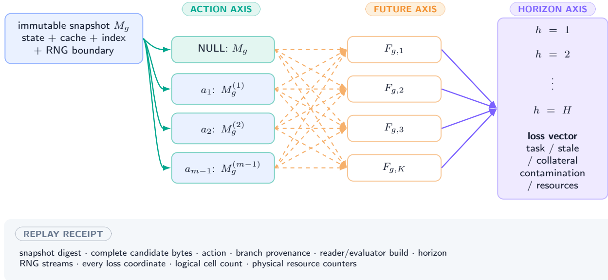
Figure 38: Action-conditioned replay tensor (DEFINITION / training only). Every feasible write and NULL starts from one immutable snapshot, is evaluated on every grouped future, and contributes all registered horizon terms. The visible |\mathcal{A}| \times K \times H lattice is logical work even when kernels batch it.
