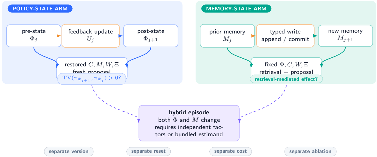
Figure 18: Mutable policy state versus external memory and workspace (DEFINITION). The navy state-swap holds context, memory, workspace, the policy-read closure, auxiliary state, and randomness fixed and asks whether a fresh proposal distribution changes. Teal memory swaps test retrieval-mediated effects separately. If the closure cannot be held fixed, the navy contrast is a bundled \Psi effect. Each state type needs its own version, reset, cost, and ablation receipt.
