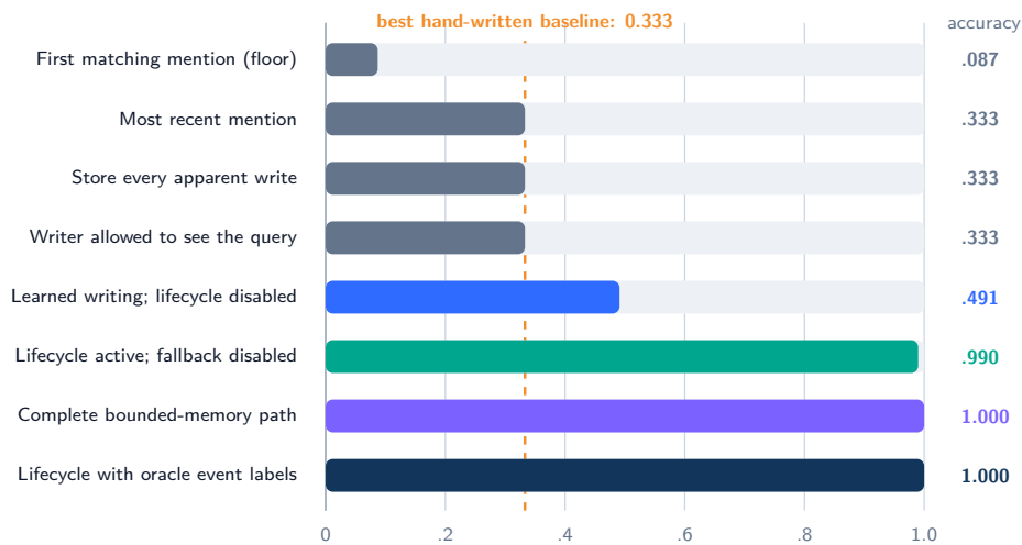
Figure 8: Held-out exact match in the controlled lifecycle study, averaged over three fixed seeds. The dashed line is the strongest hand-written rule. Under the registered implementation and training recipe, the complete typed lifecycle path outperforms the specified lexical baselines and component-removal controls; disabling lifecycle execution roughly halves accuracy, while disabling fallback loses only the capacity-pressure cases.
