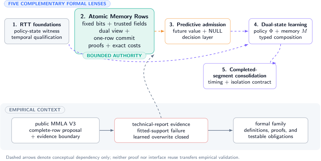
Figure 1: Atomic rows occupy the bounded substrate layer of a five-paper conceptual family. Dependency arrows organize formal interfaces; they do not transfer empirical validation. The semantic-interface and learned-overwrite gates remain closed.
