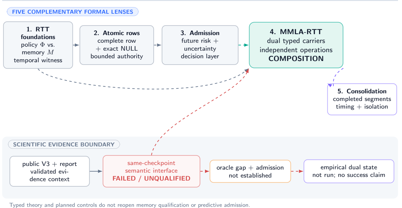
Figure 1: Dual-state composition in the five-paper conceptual family. The semantic-interface stop is inherited and remains closed; formal prerequisites do not provide empirical validation.
