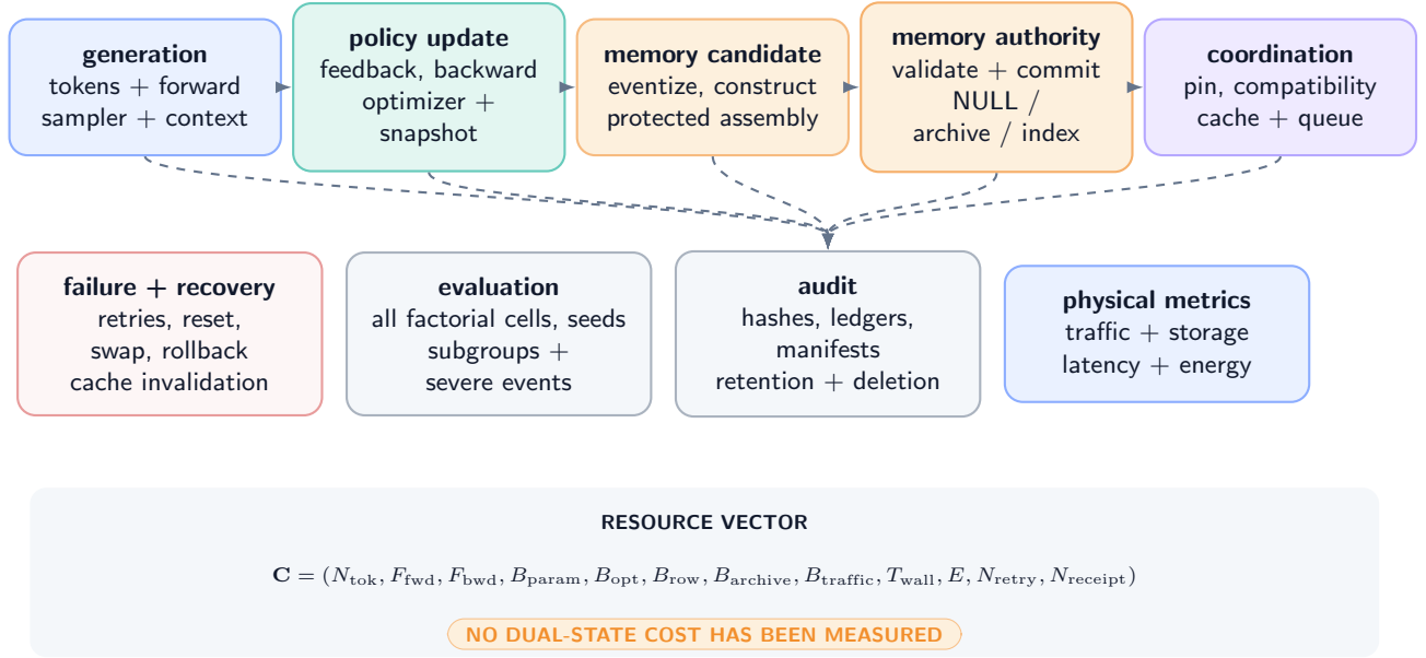
Figure 9: Training, reasoning-time, memory, recovery, and audit ledgers (DEFINITION / DESIGN PRESCRIPTION) . Parallelism may reduce wall time but cannot delete logical work, bytes, validation, or failed attempts from the ledger.
