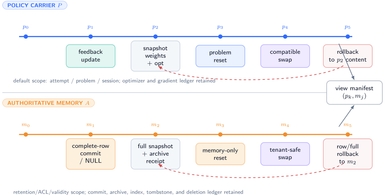
Figure 4: Independent lifetimes, snapshots, rollback domains, and ledgers (DESIGN PRESCRIPTION). A view manifest can name both carrier versions; it cannot collapse their lineages or authorize silent cross-restoration.
