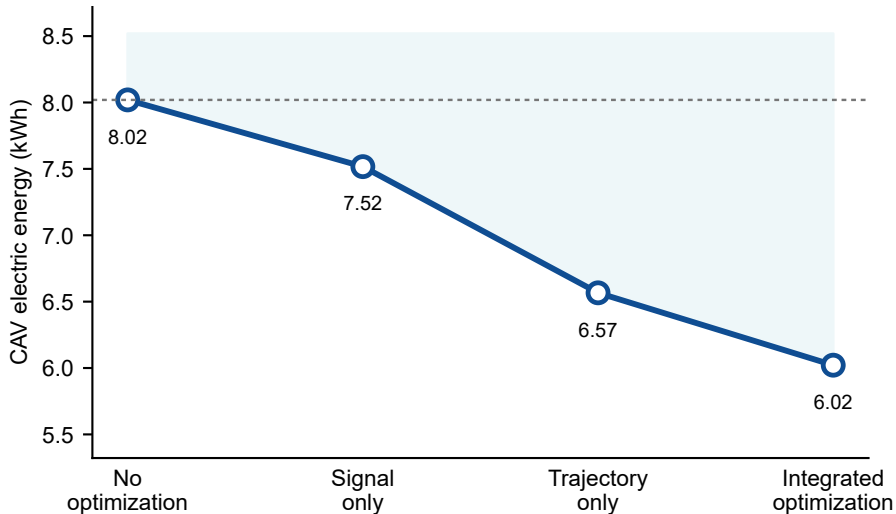
CAV energy use across scenarios
