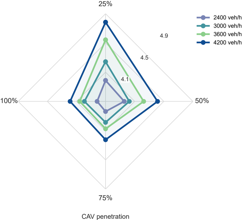
CAV jerk over traffic volume and CAV penetration
