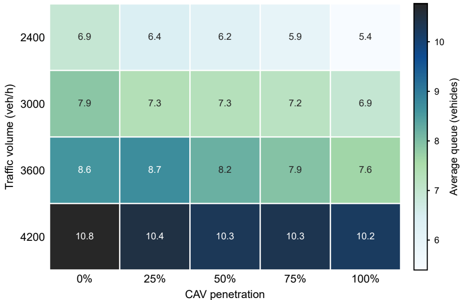
Queue length over traffic volume and CAV penetration
