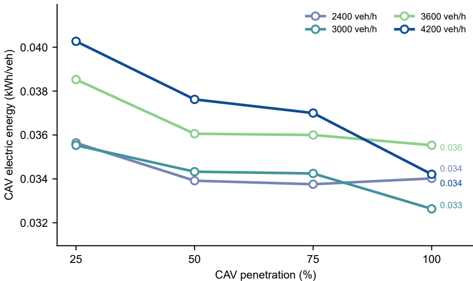
CAV energy use over traffic volume and CAV penetration
