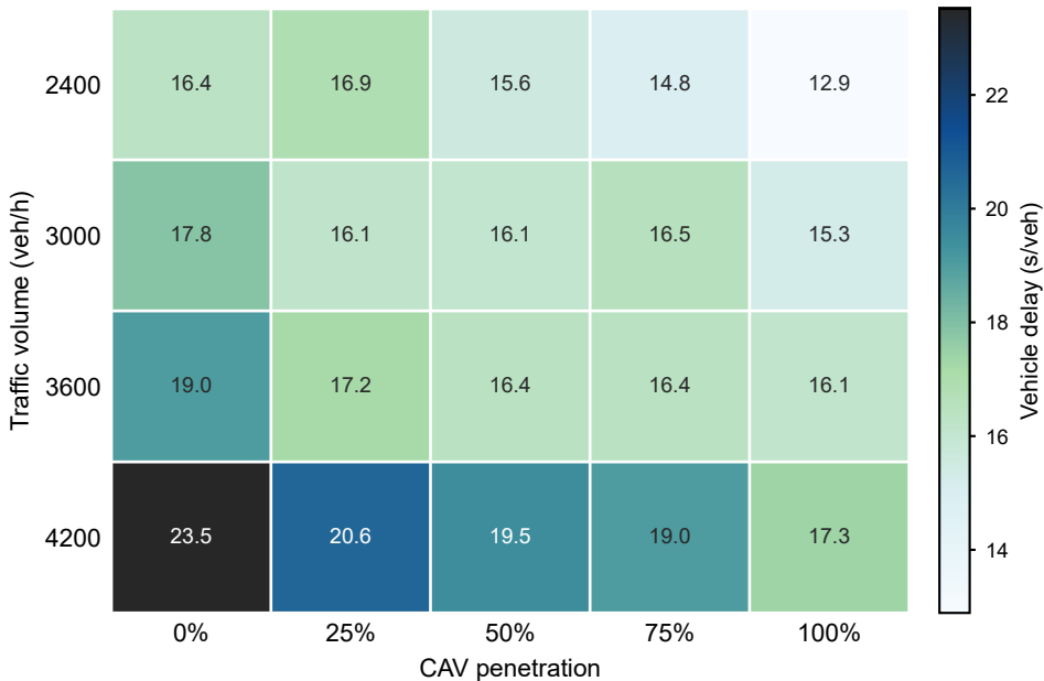
Delay over traffic volume and CAV penetration
