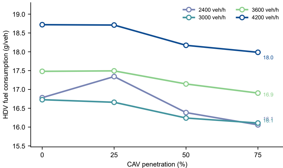
HDV fuel use over traffic volume and CAV penetration
