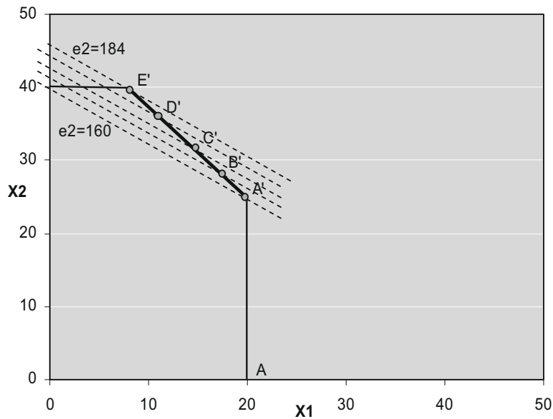
Fig. 3. Results of the \varepsilon -constraint method from model using lex-optimization in the payoff table. New
