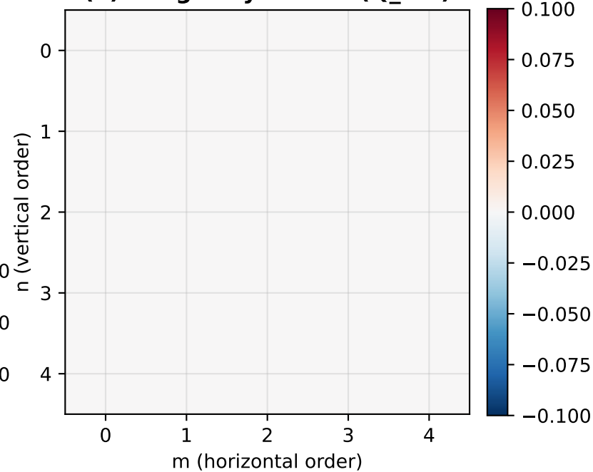
(e) Imaginary Part \text{Im}(Q_{nm})
