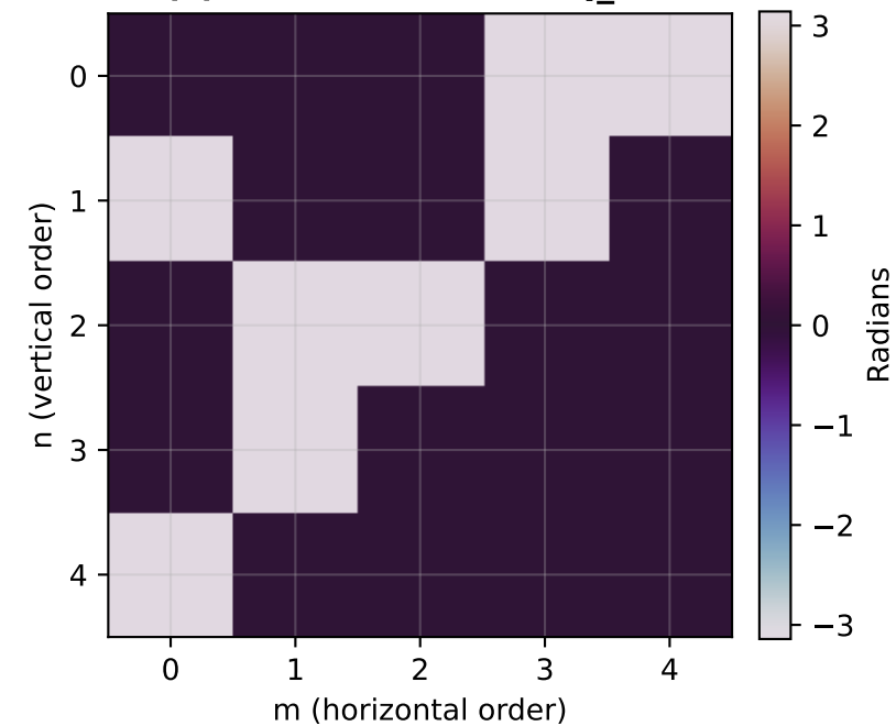
(c) Moment Phase \angle Q_{nm}
