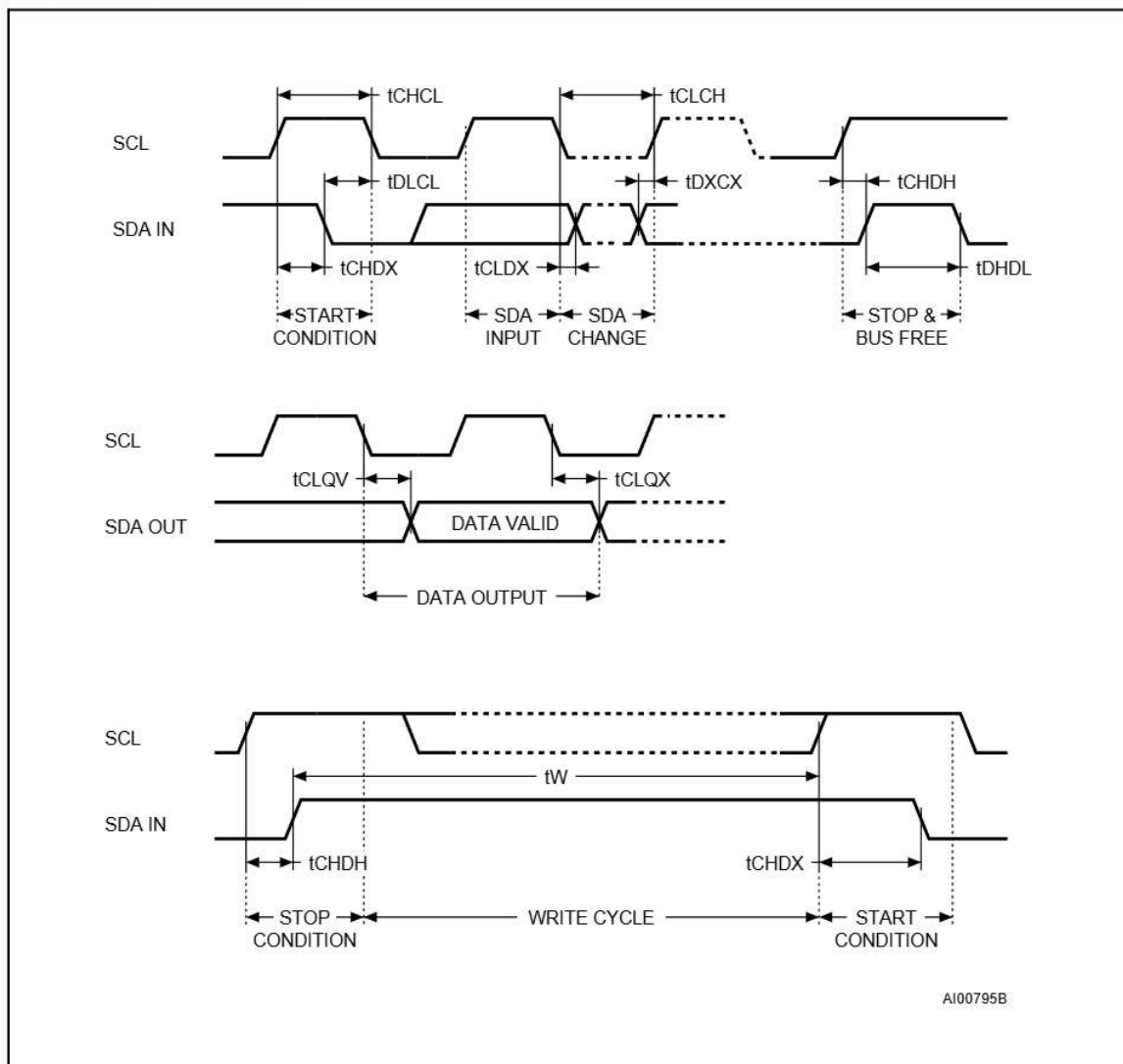
Figure 5. AC Waveforms
