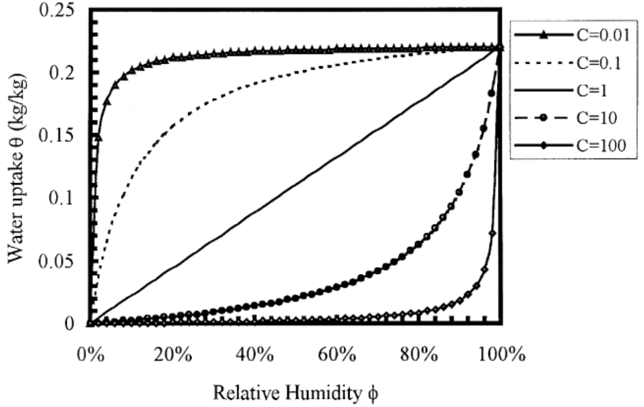
Fig 2: Sorption curves with representative C numbers.
