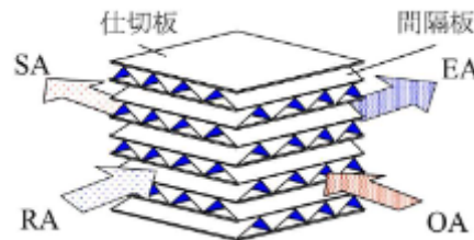
図 1: Schematic of a enthalpy exchanger element (corrugate/ cross flow) .
